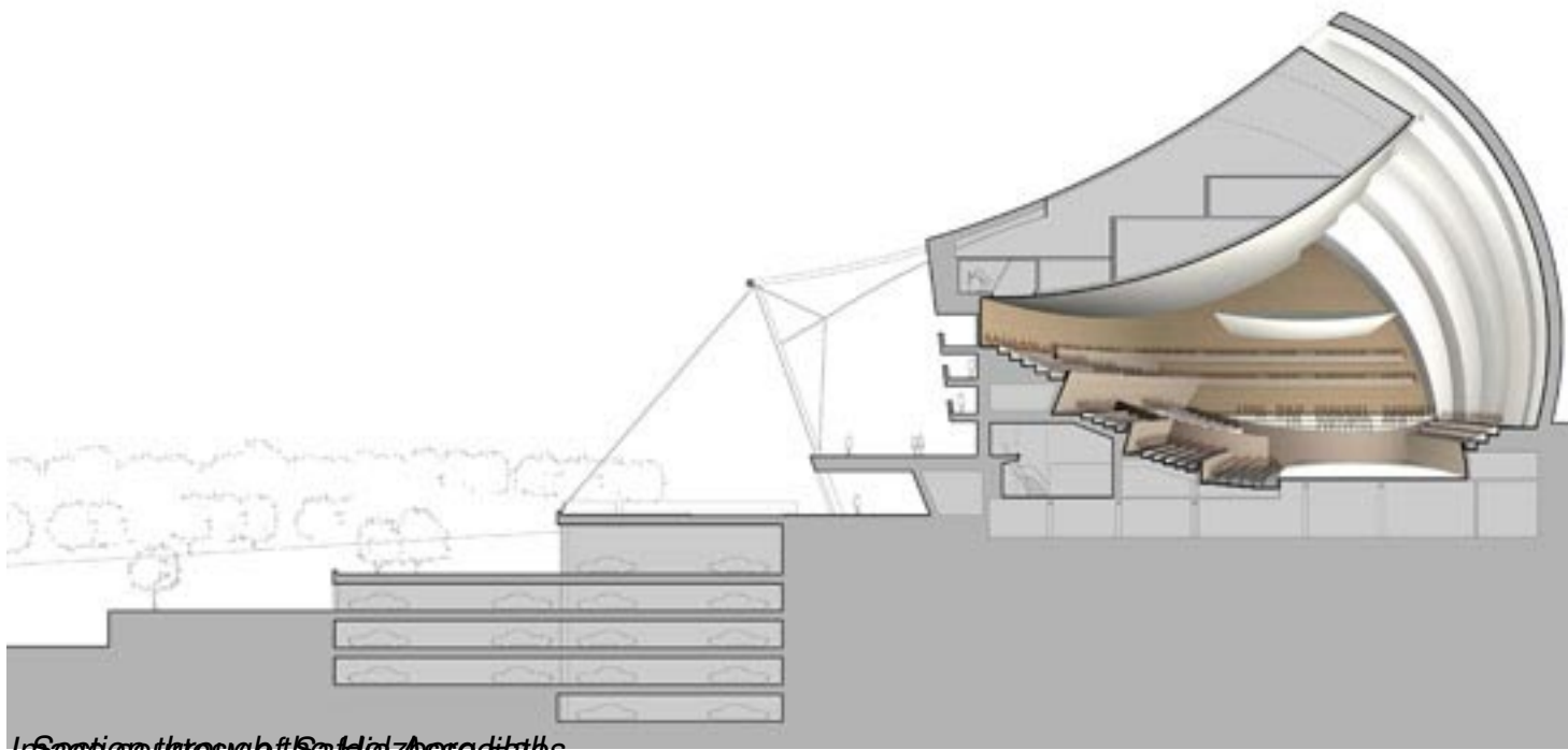
Section through the Solid Amphitheater
