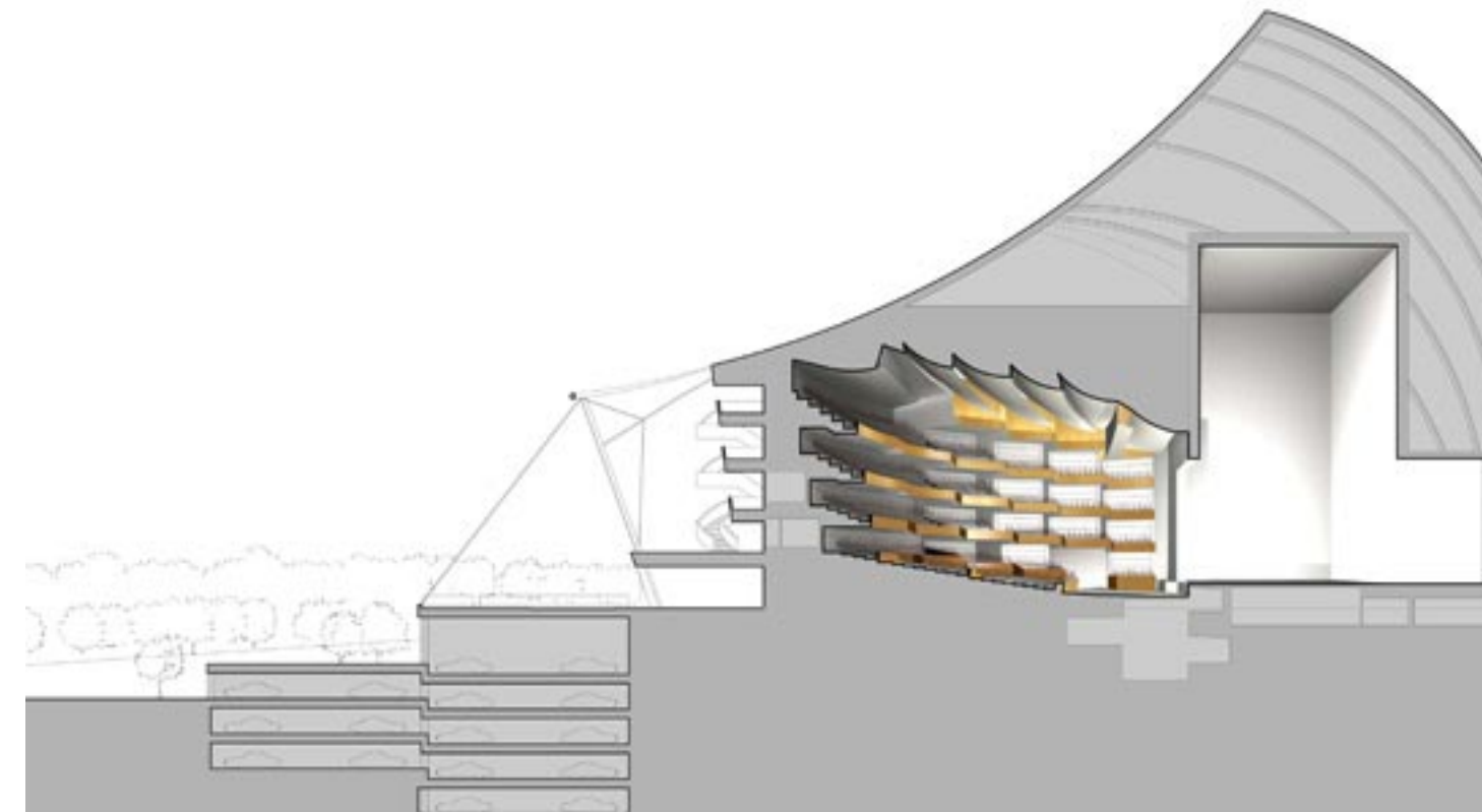
Section through the Solid Amphitheater
