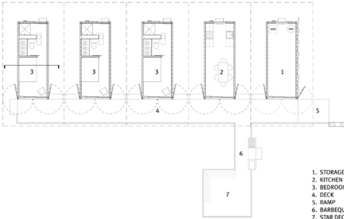
FLOOR PLAN
