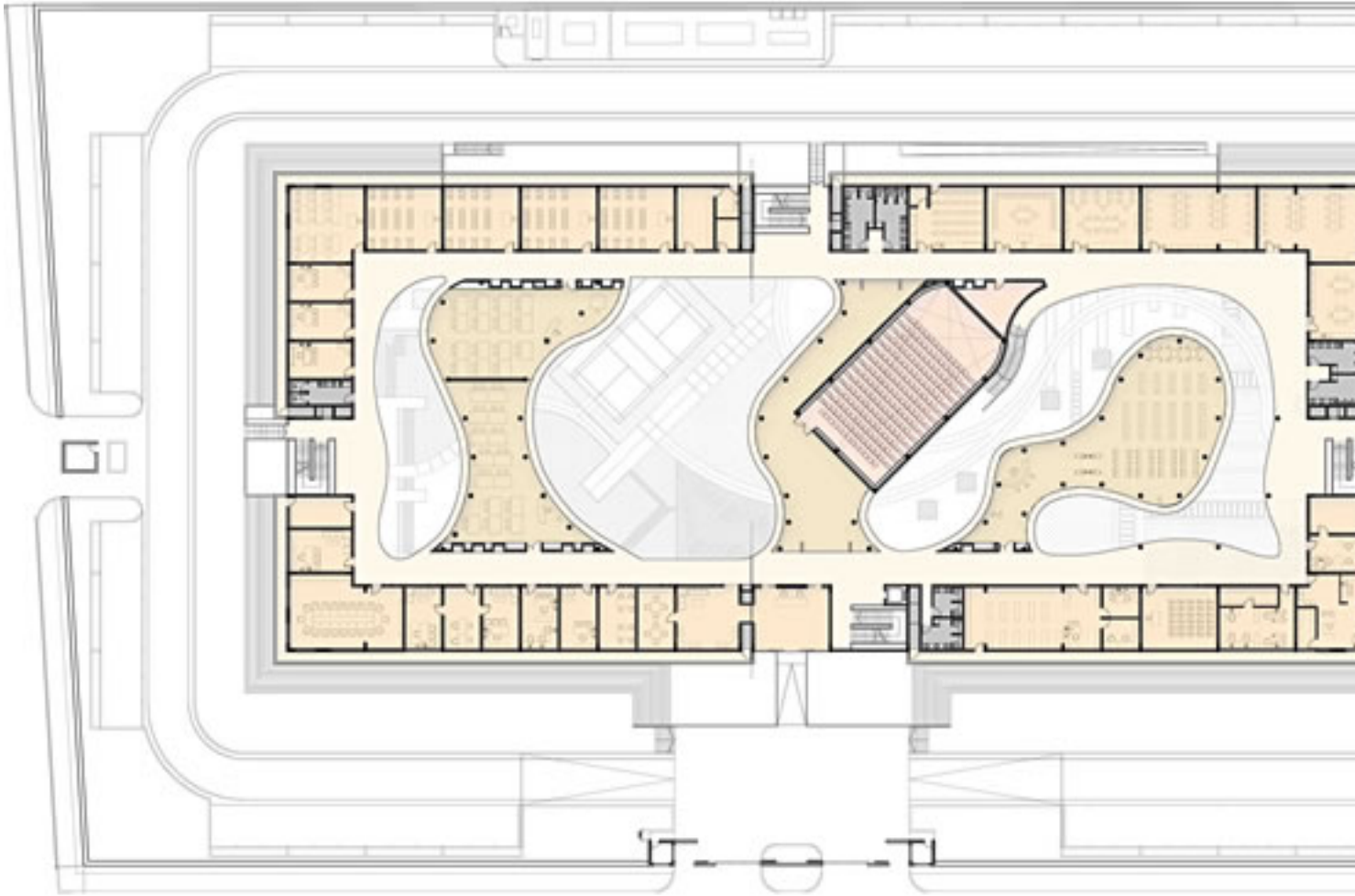
Plan
